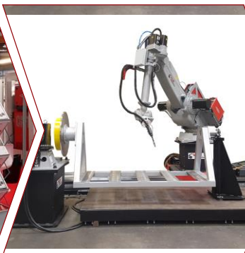
manufacturing cell additive metal parts > 5 m (Polyshape)
