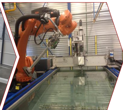
NDT cell for control of A350 structural composite parts (Stélie, Airbus Group)
