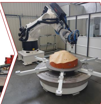
multifunctional machining cell for composite (Nimitech, Lauak)
